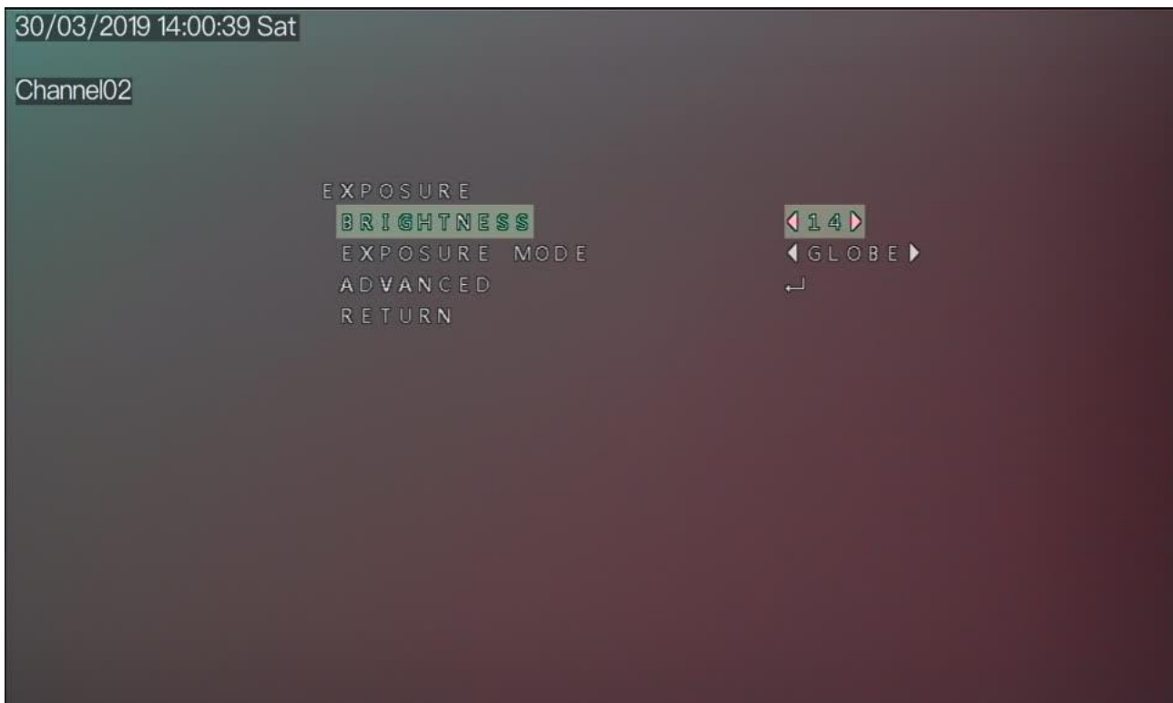
Figure 2-1 EXPOSURE interface
