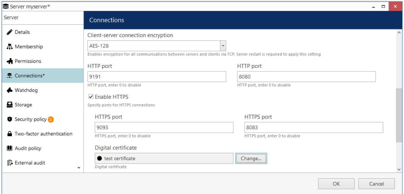
Ganz CORTROL Global server connection settings with encryption options
