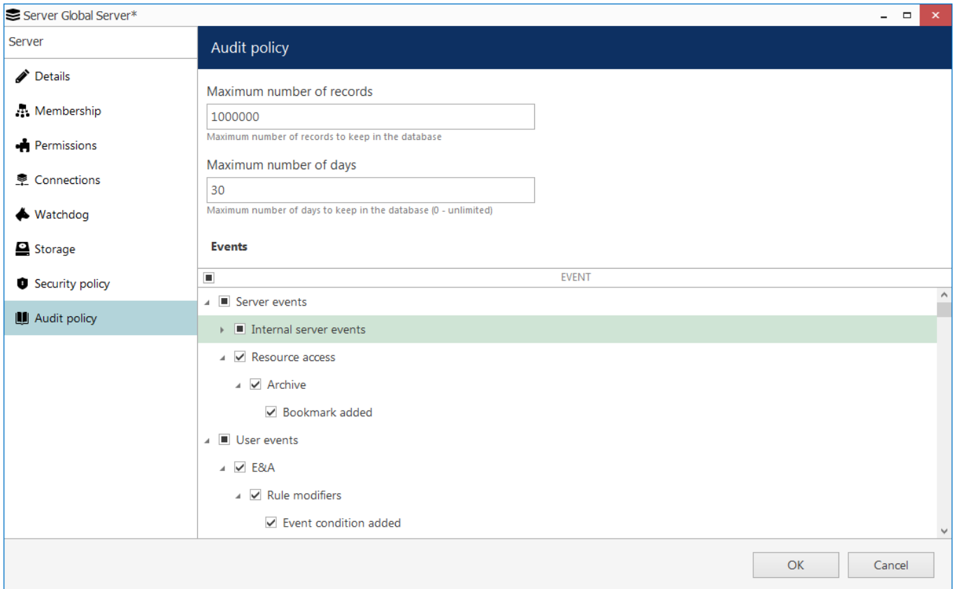
Ganz CORTROL audit policy
