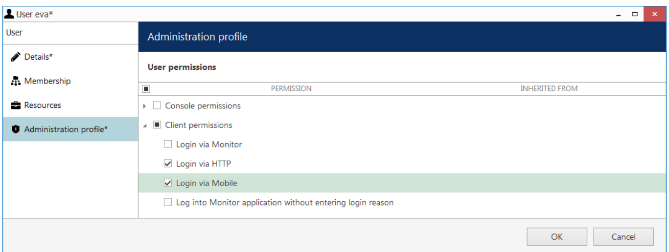
User permissions for Ganz CORTROL Mobile and Web browser login
